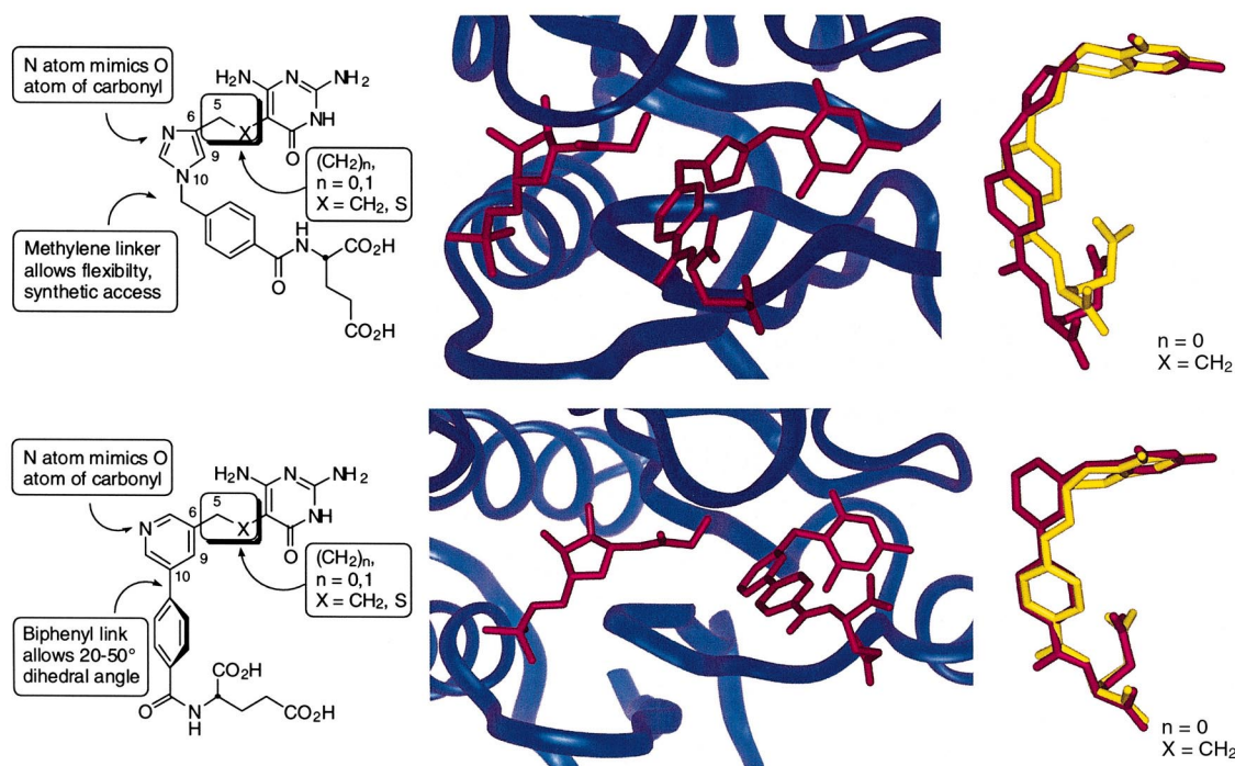
Figure 3. Models of 3 (brown, top; n=0 , X=\text{CH}_2 ) and 4 (brown, bottom; n=0 , X=\text{CH}_2 ) bound in the GAR Tfase active site and structural overlays with the structure of 5,10-dideazatetrahydrofolate (yellow) taken from the X-ray crystal structure bound to GAR Tfase. 28
